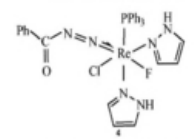
[ReClF(CO)(Cl)(PPh 3 )]
