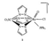
[ReOCl(CO)(C(=O)PPh 3 )]
