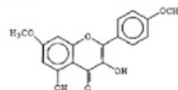
I 3,5-DIHI-DROXI-4',7-DIMETOXI-FLAVONA
