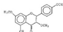
II 5-HI-DROXI-3,4',7-TRI-METOXI-FLAVONA
